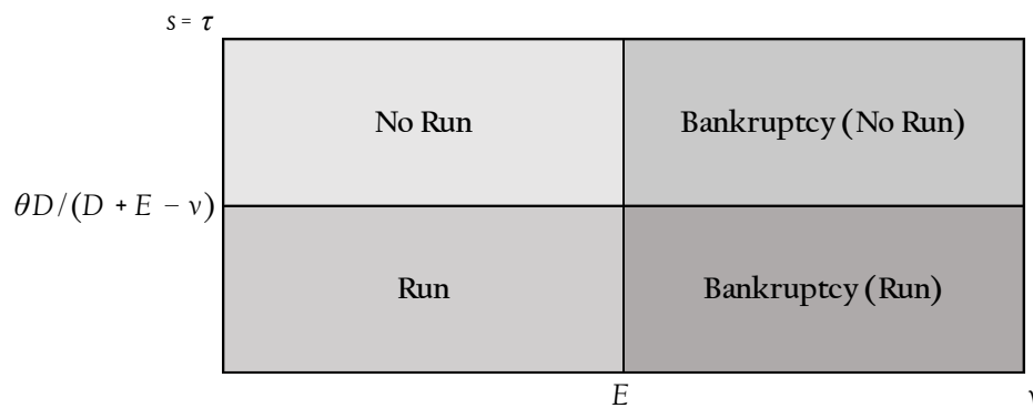
Figure 1: Possible Equilibria
